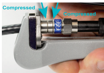
Compressing PCT-TRSXL-6L or PCT-TRSXL-6LMG Connectors
