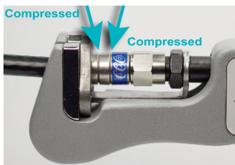
Compressing PCT-TRS-6L or PCT-TRS-6LMG Connectors
